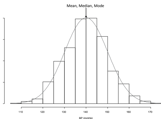
Figure 1. Normal distribution
